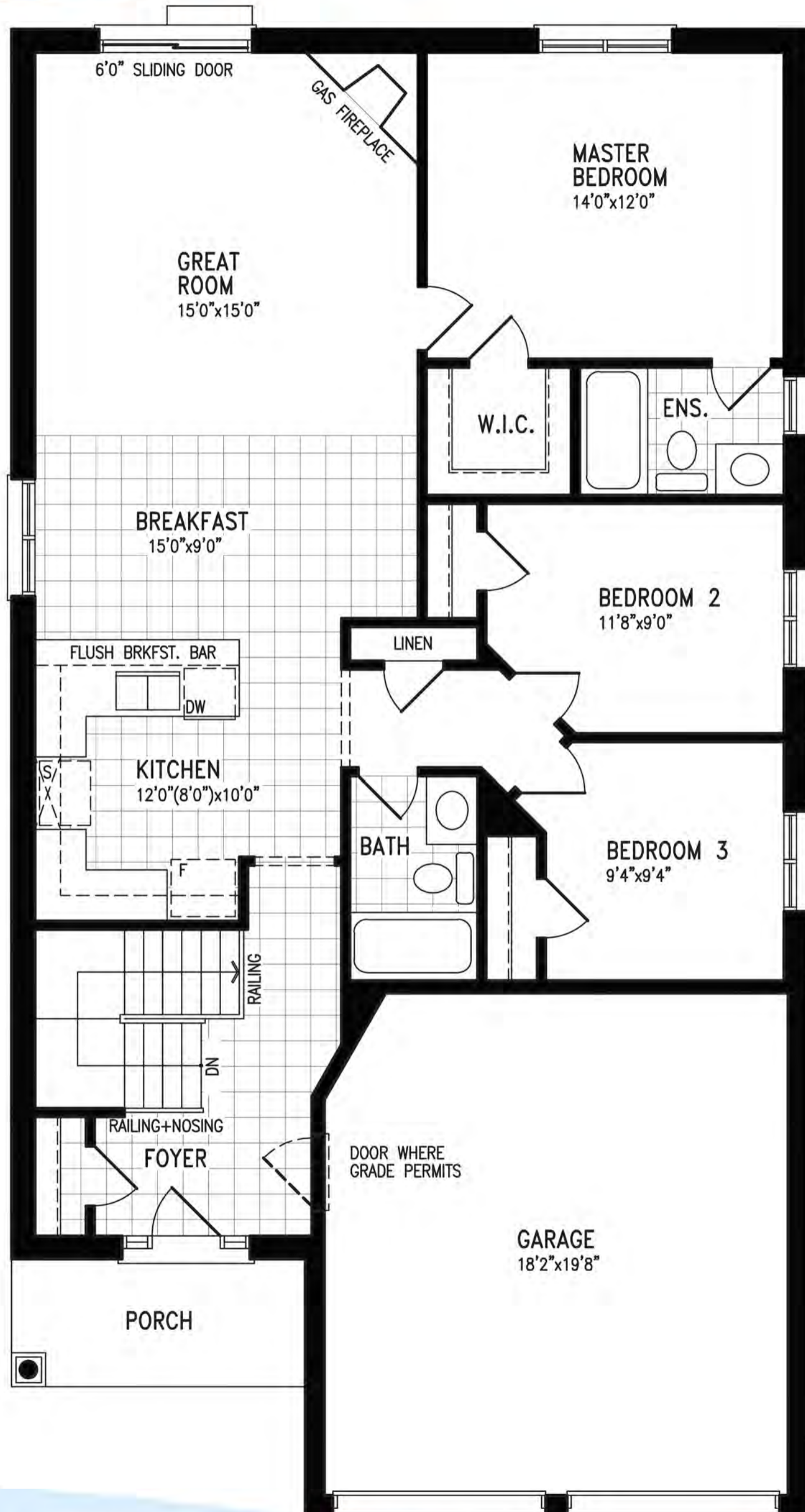
GROUND FLOOR PLAN 'A' - 3 BEDROOM
