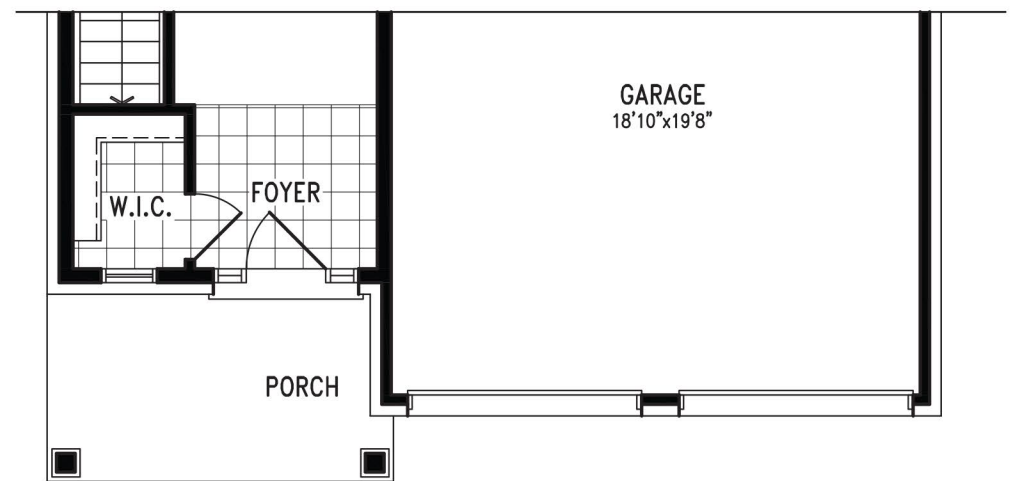
Partial Ground Floor Plan 'B'
