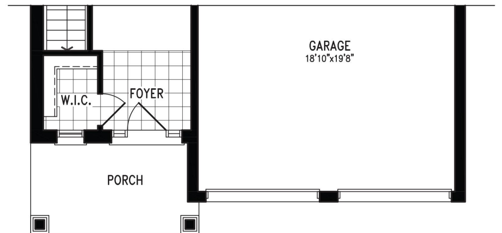
Partial Ground Floor Plan 'C'
