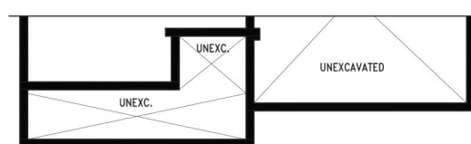
Partial Basement Floor Plan 'B'
