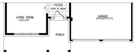
Partial Ground Floor Plan 'B'
