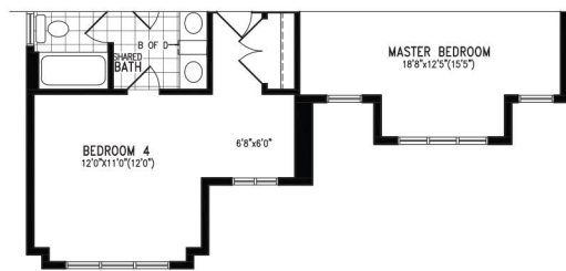
Partial Second Floor Plan 'B'
