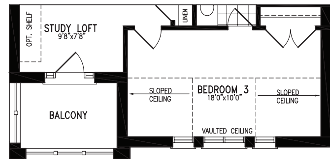
Partial Second Floor Plan 'C'
