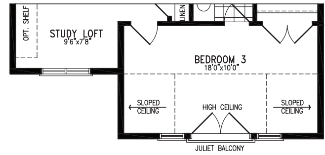
Partial Second Floor Plan 'B'
