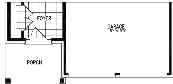
Partial Ground Floor Plan 'B'
