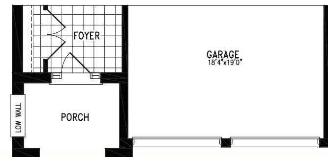
Partial Ground Floor Plan 'C'
