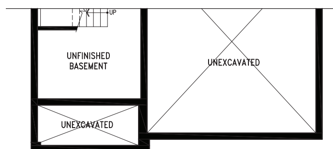
PARTIAL BASEMENT PLAN 'B'
