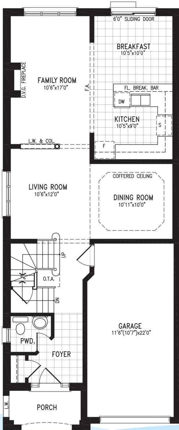
GROUND FLOOR PLAN 'A'
