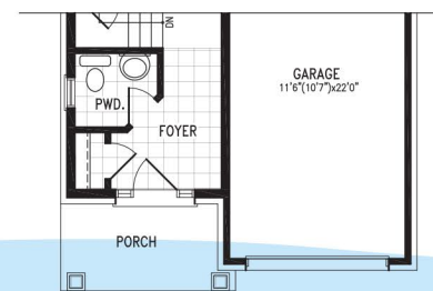
PARTIAL GROUND FLOOR PLAN 'B'
