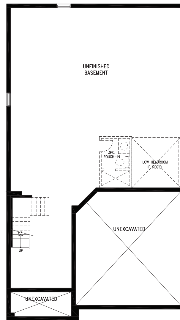
BASEMENT FLOOR PLAN 'C'
