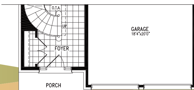
PARTIAL GROUND FLOOR PLAN 'A'
