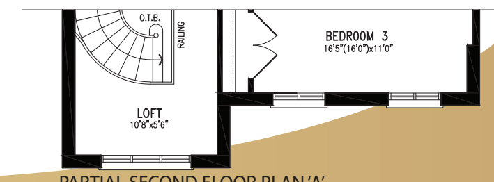
PARTIAL SECOND FLOOR PLAN 'A'
