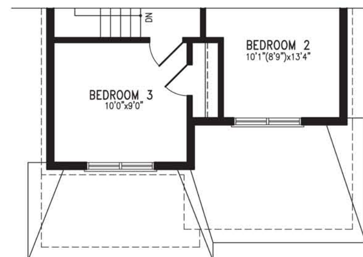
PARTIAL SECOND FLOOR PLAN 'B'
