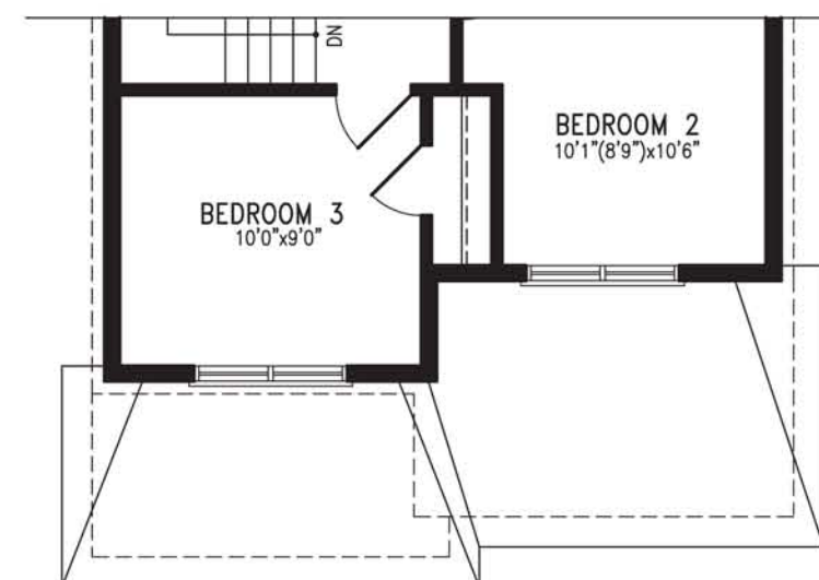
OPT. PARTIAL SECOND FLOOR PLAN 'B' WITH UPGRADED ENSUITE
