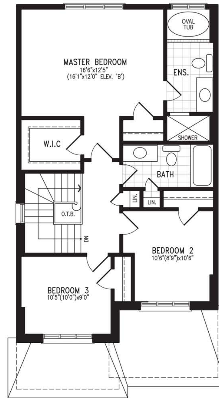
OPT. SECOND FLOOR PLAN 'A' WITH UPGRADED ENSUITE
