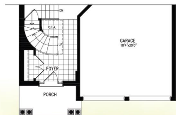
Partial Ground Floor Plan 'A'
