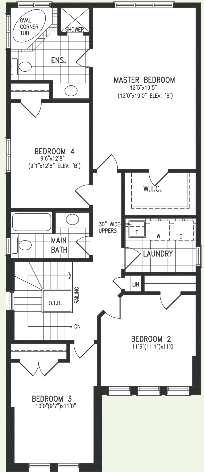
SECOND FLOOR PLAN 'A'
