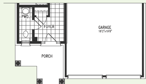
PARTIAL GROUND FLOOR PLAN 'B'
