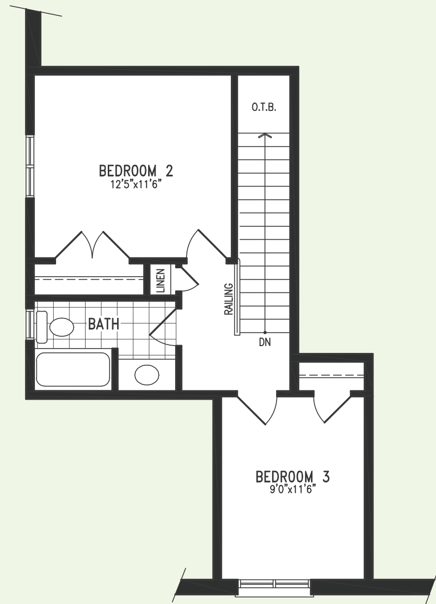
LOFT FLOOR PLAN 'A'
