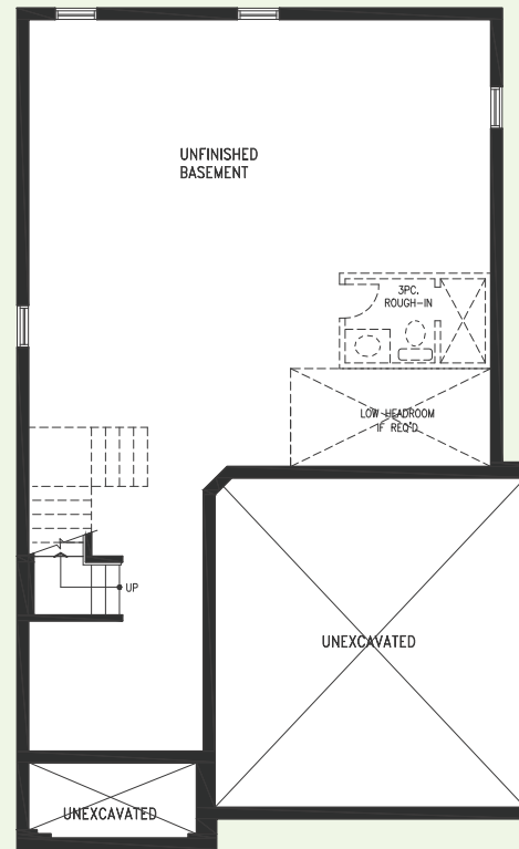
BASEMENT PLAN 'A' / 'C'
