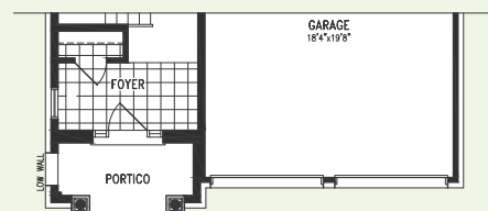
PARTIAL GROUND FLOOR PLAN 'B'
