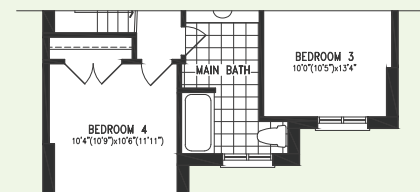
PARTIAL SECOND FLOOR PLAN 'A'
