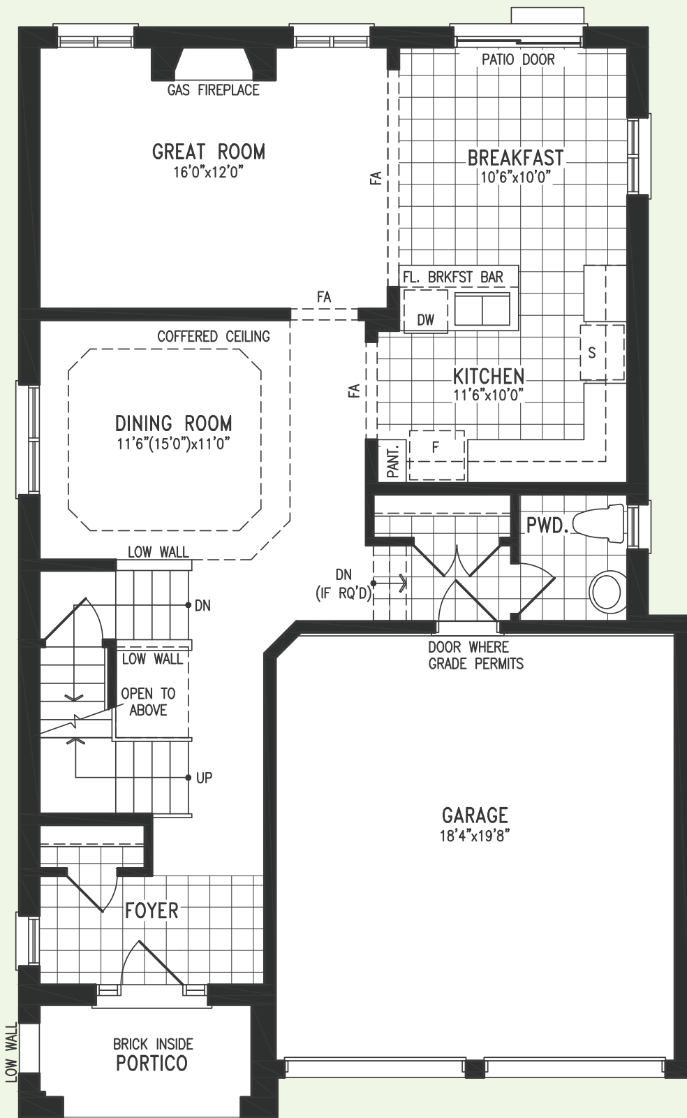
GROUND FLOOR PLAN 'C'
