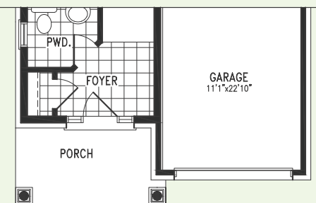
PARTIAL GROUND FLOOR PLAN 'B'
