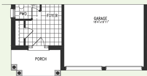
PARTIAL GROUND FLOOR PLAN 'A'
