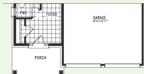
PARTIAL GROUND FLOOR PLAN 'B'
