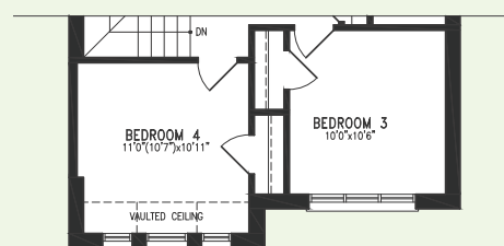
PARTIAL SECOND FLOOR PLAN 'A'
