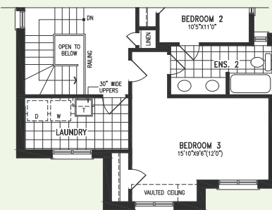
PARTIAL OPT. SECOND PLAN 'A' W/ 3 BATH
