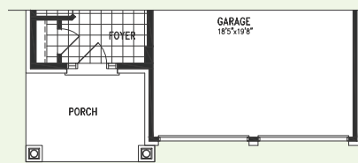
PARTIAL GROUND FLOOR PLAN 'B'
