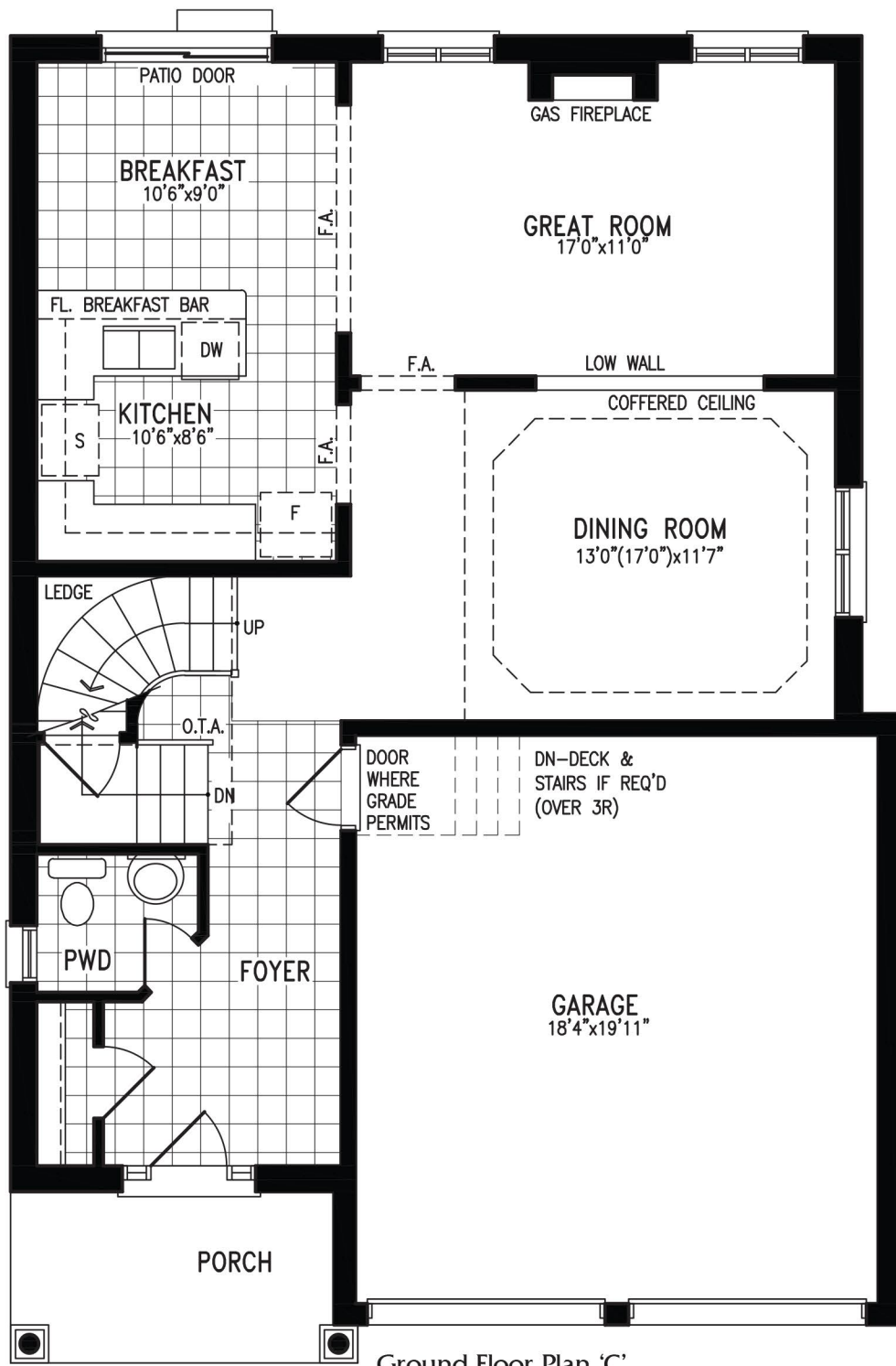
Ground Floor Plan 'C'
