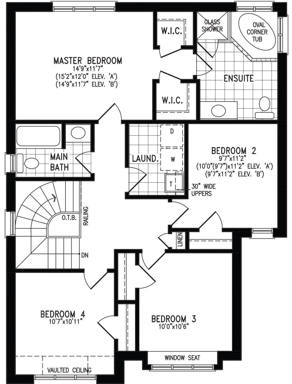
Second Floor Plan 'C'
