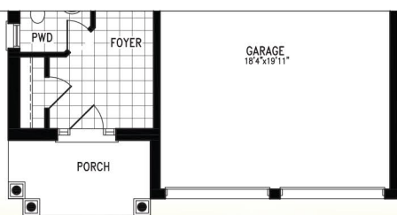
Partial Ground Floor Plan 'A'
