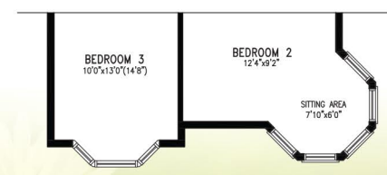
Partial Second Floor Plan 'B'
