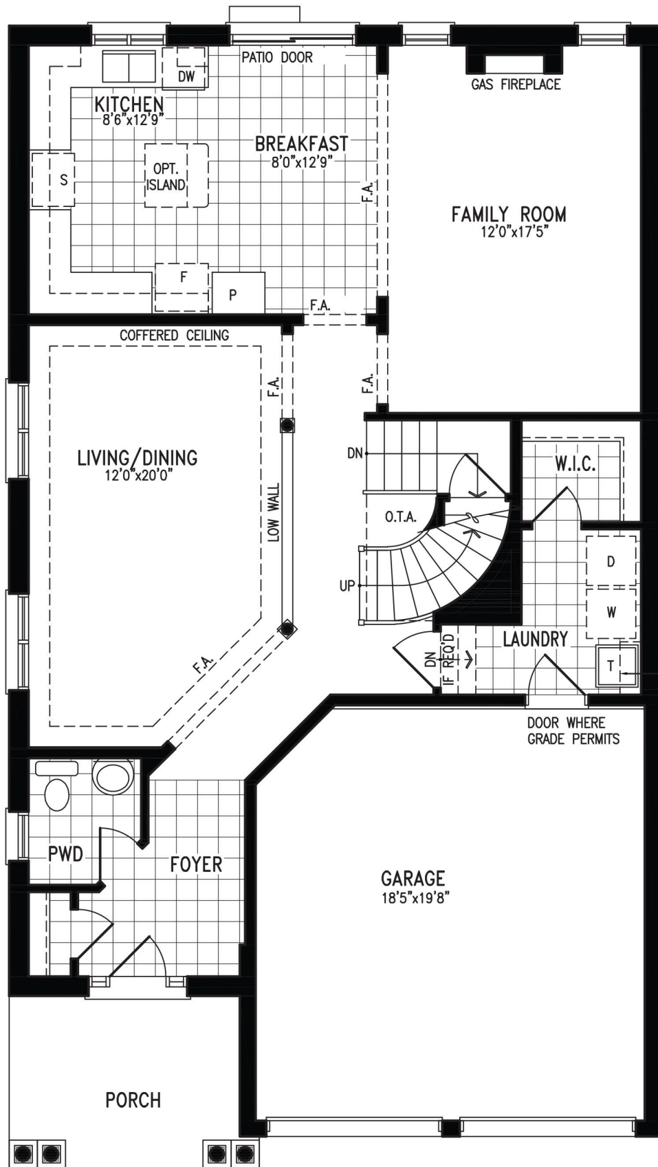
Ground Floor Plan 'C'
